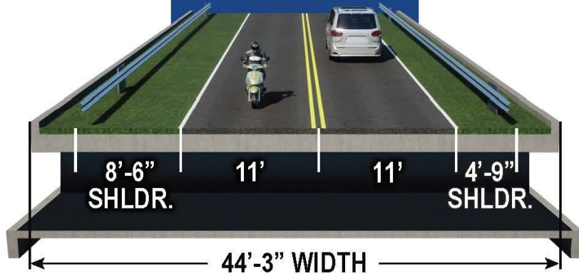
Existing Bridge
